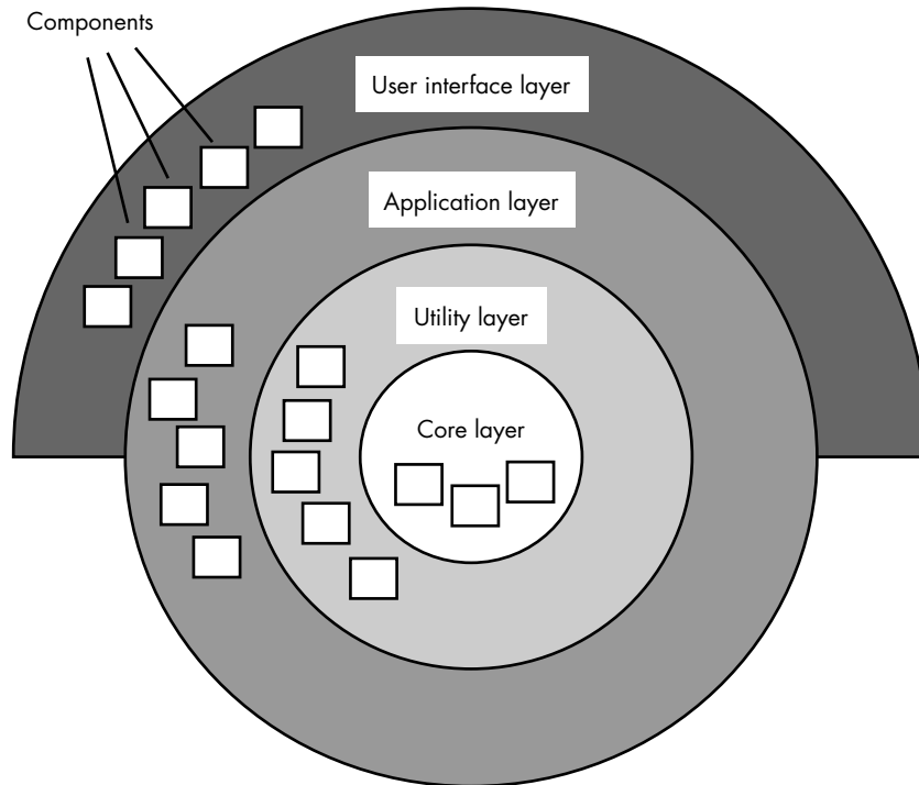
FIGURE 14.3 Layered architecture
